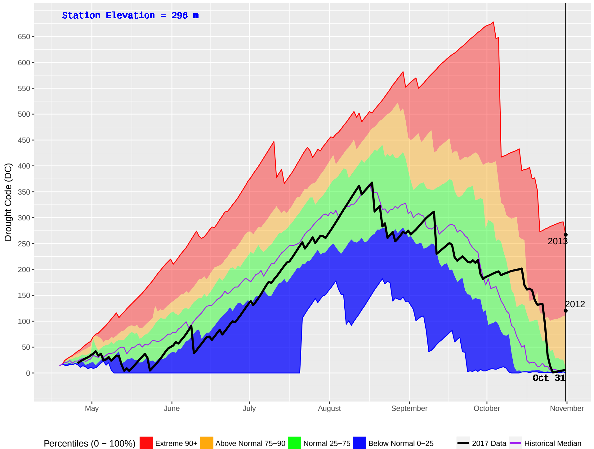
VAN DYKE (430) : Historical (1983–2016) and Current (2017) Noon Drought Code (DC)
