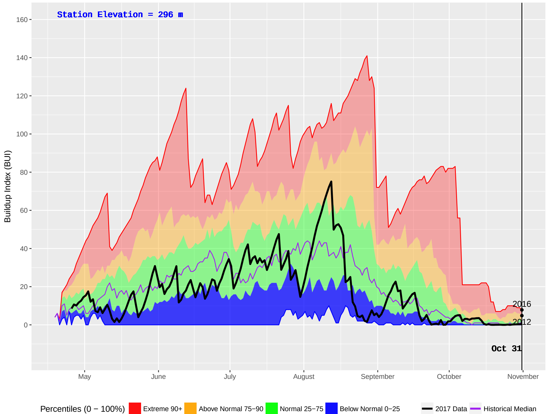
VAN DYKE (430) : Historical (1983–2016) and Current (2017) Noon Buildup Index (BUI)
